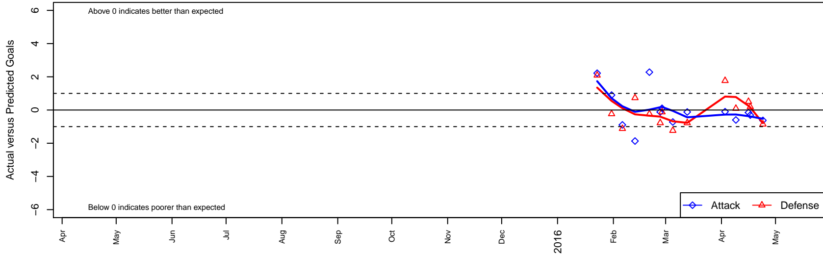
Capital FC Timbers Black G99 Dots are actual minus expected GF (blue circles) and GA (red triangles). Blue line is smoothed change in attack strength. Red is smoothed change in defense strength.
